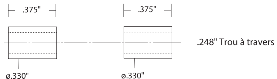
Figure C / Collets #PKM-BUSH3
